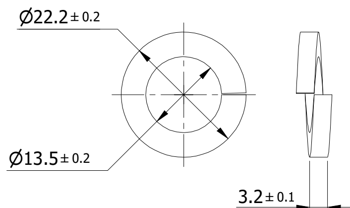
1/2" SPRING WASHER SS
