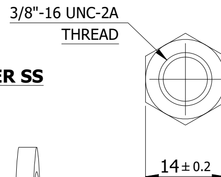
3/8"-16 UNC-2A NUT SS
